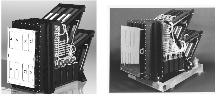
Figure 2. Left: CAD illustration of the SMM/Bent Crystal Spectrometer with channel numbers indicated. Right: The instrument bolted to a calibration jig prior to installation in the SMM spacecraft. The heat shield can be seen mounted on the instrument front face (to the left). The analogue-signal-processing electronics, digital electronics, and power supplies were mounted elsewhere in the spacecraft and are not shown. The instrument height was 580 mm and width 350 mm.
