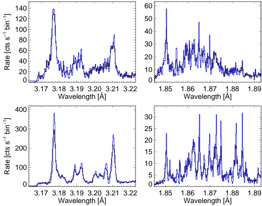
Figure 14. Channel 1 (upper left) and channel 4 (upper right) spectra are shown for the rising phase (09:17–09:18 UT) of a flare on 10 April 1980 (SOL1980-04-10T09:22). The black histograms are the raw data and the blue histograms are the deconvolved data. The flare rise phase coincides with a hard X-ray peak; broadened lines and extra emission on the short-wavelength side (“blue shifts”) of all lines are evident. Equivalent spectra are shown (lower left and lower right) for the flare’s post-peak (09:27–09:28 UT), when the blue shifts are no longer apparent.
