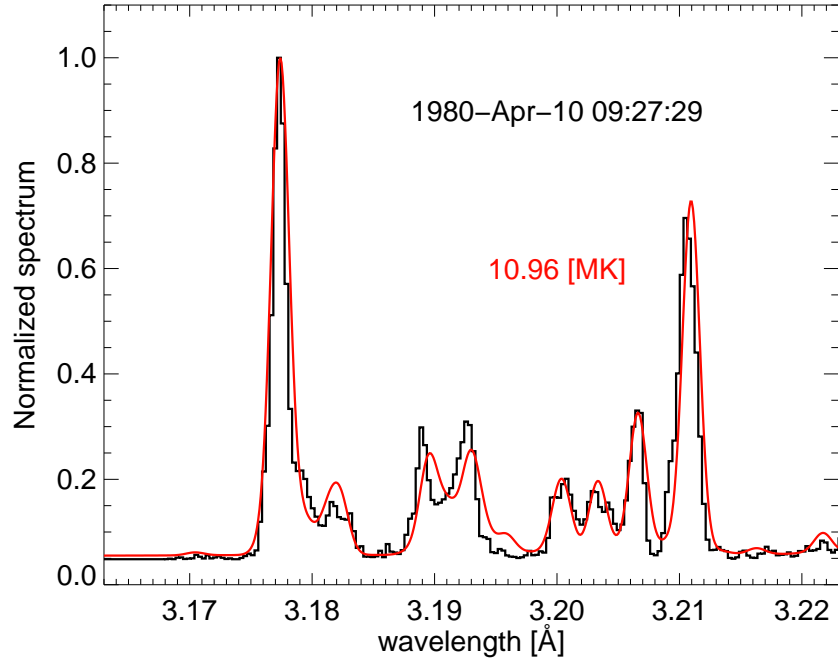
Figure 15. BCS spectrum during the decay of the flare of 10 April 1980 (SOL1980-04-10T09:22) fitted with the synthetic spectrum program described in the text for an electron temperature of 10.96 MK. Spectrum is normalized to the Ca XIX w line at 3.177 Å.
