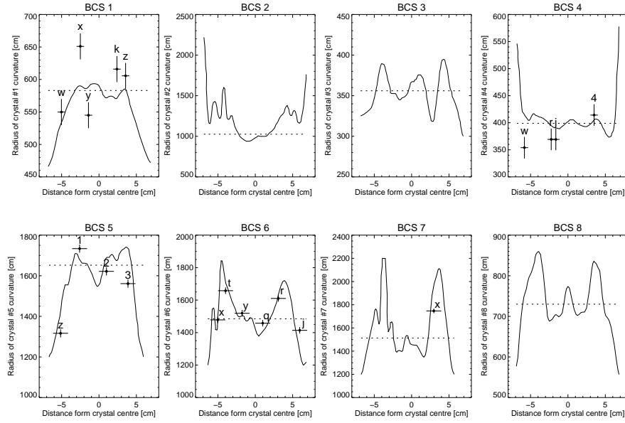
Figure 3. Radius-of-curvature measurements (solid curves) made during the qualification of the eight BCS crystals (channel numbers are indicated above each plot). The crosses indicate radius measurements made using spectral lines in each channel (notation of Gabriel (1972)) during the spacecraft raster of 06 November 1980. The nominal (design) curvature for each crystal is shown as a dotted horizontal line in each panel. Figure adapted from Parmar (1981).
