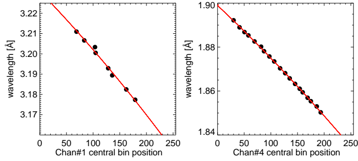
Figure 7. Bin number of the peak of prominent spectral lines versus line wavelength for BCS channels 1 (left) and 4 (right) during the 01 July 1980 flare (SOL1980-07-01T16:28) to illustrate the near-linearity of these channels during the 1980 Mission. The spectral lines include those shown in Figure 4.
