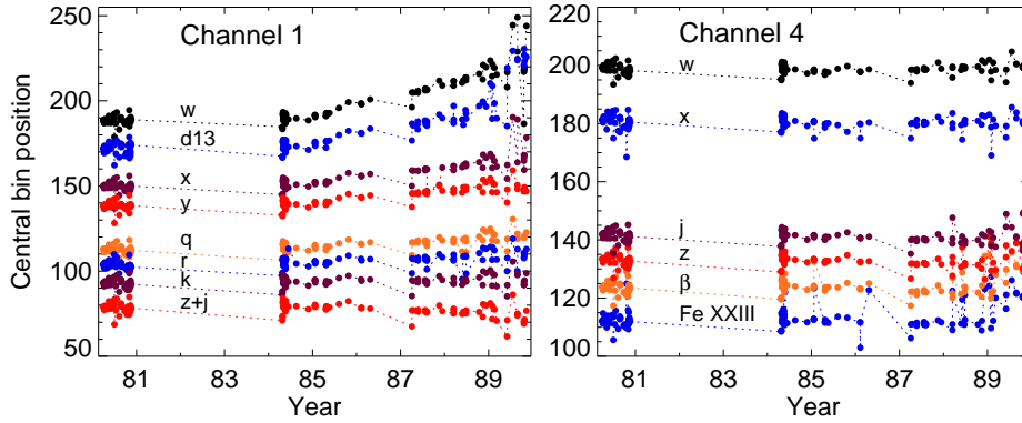
Figure 4. Left panel: Fitted bin positions of Ca XIX line w and other lines in BCS channel 1 versus time over the lifetime of SMM. Right panel: Corresponding data for Fe XXV line w and other lines in channel 4. (Line notation follows Gabriel (1972).)
