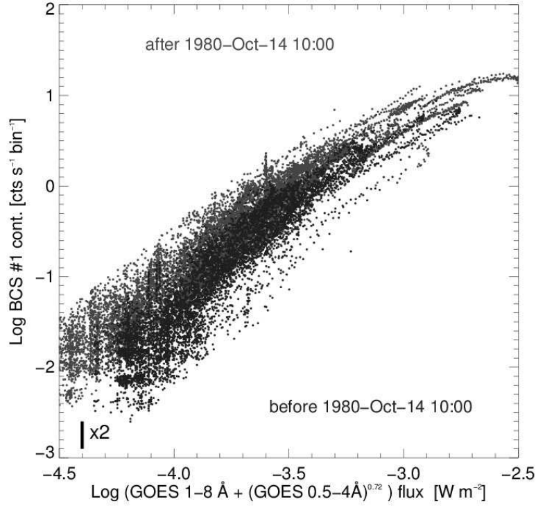
Figure 11. Flux in a line-free portion of Channel 1 ( 3.168\text{--}3.171\text{ \AA} ) shown on a log-log plot versus GOES fluxes in the form \text{GOES}(1\text{--}8\text{ \AA}) + \text{GOES}(0.5\text{--}4\text{ \AA})^{0.72} for flares before (dark grey) and after (light grey) 14 October 1980 (10:00 UT). The scatter is due to the lower BCS collimator transmission for flares occurring off-axis. The upward shift between the dark and light grey points by approximately a factor 2 (indicated by the black vertical bar, lower left) is apparent, and is attributed a sensitivity increase through the loss of the Second Surface Mirror (SSM). [Journal version will be in colour.]
