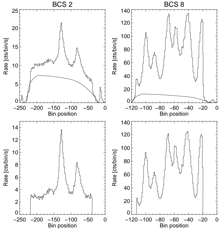
Figure 13. Analysis by Parmar (1981) of spectra in BCS channels 2 (left panels) and 8 (right panels) in which fluorescence emission, modeled with a Monte Carlo routine (smooth curves in upper panels), is removed to give the corrected spectra in the lower panels.
