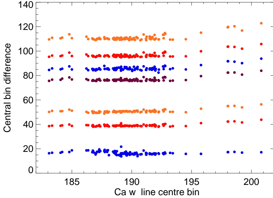
Figure 8. Distances (in bins) between bin zero and various Ca XIX lines and Ca XVIII satellites for 102 flares recorded over a wide range of offsets by the BCS before 01 January 1987. Points are colour-coded for lines observed in channel 1 – blue: line w and d13 ; red: w and x ; orange: w and y ; violet: w and q ; blue: w and r ; red: w and k ; orange: w and z (blended with j ). (Line notation is from Gabriel (1972).)
