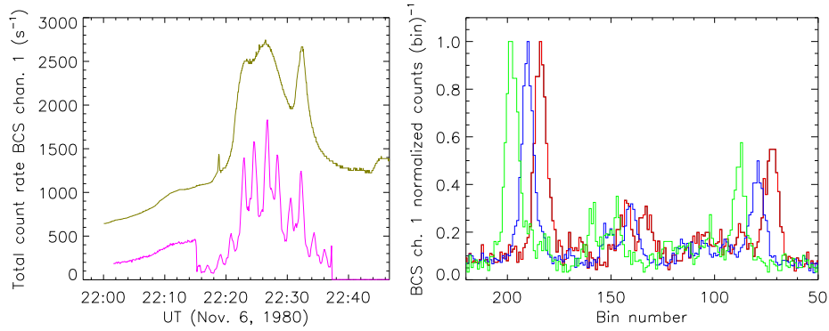
Figure 5. Left panel: BCS light curve (in magenta: total counts \text{s}^{-1} , channel 1) during the spacecraft scans of 06 November 1980 (22:15–22:37 UT) when an M3.5 flare (SOL1980-11-06T22:27) was in progress; modulations are due to the flare repeatedly passing through the BCS collimator response. Normalized GOES (0.5–4 Å) light curve plotted in olive. Right panel: Normalized BCS channel 1 spectra plotted against bin number at 22:23:48 UT (red), 22:24:39 UT (blue), and 22:25:36 UT (green), illustrating the shift of spectra against bin number for when the flare was along the BCS boresight (blue) and at each end of the spacecraft manoeuvre range (red and green). The accumulation time for each spectrum was 6 seconds, and the angular range of the spacecraft scans was \pm 3.5 arcmin in the BCS dispersion direction.
