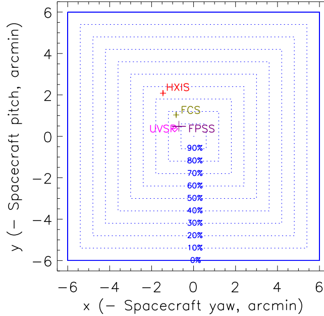
Figure 12. BCS collimator response in spacecraft coordinates (x, y) shown as squares (dashed lines) with collimator response in percentages of the peak (central) value. Also shown are the boresight positions (with estimated uncertainties) of the spacecraft FPSS (purple), the FCS (dark green: see text) and HXIS (red) instruments. The UVSP boresight is indicated (magenta diamond) but no uncertainties are available. The boresight positions are based on 1980 flare data (Waggett, 1986). The BCS dispersion is in the E–W ( \pm x ) direction.
