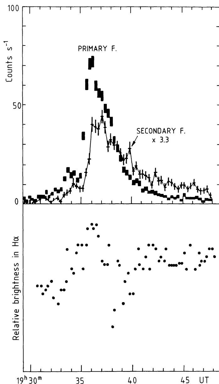
Fig. 6. Above: (HXIS): time development of the 3.5–5.5 keV X-ray emission at the primary and secondary footpoints of the flaring arch No. 23. Below (Big Bear): relative photometry of the H\alpha brightness at the secondary footpoint.
