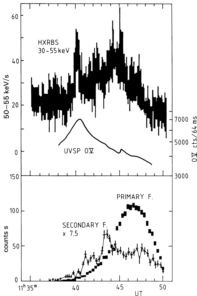
Fig. 3. Below : time developments of the X-ray flux in the energy range 3.5–5.5 keV at the two footpoints of the arch during the brightening No. 5 (HXIS). Above : time development of the total emission during this brightening in hard X-rays (Hard X-Ray Burst Spectrometer, HXRBS; Orwig, Frost, and Dennis, 1980) and in the O v line in the transition layer (Ultraviolet Spectrometer and Polarimeter, UVSP). The two upper curves have been taken from Figure 7 in Švestka et al. (1982).
