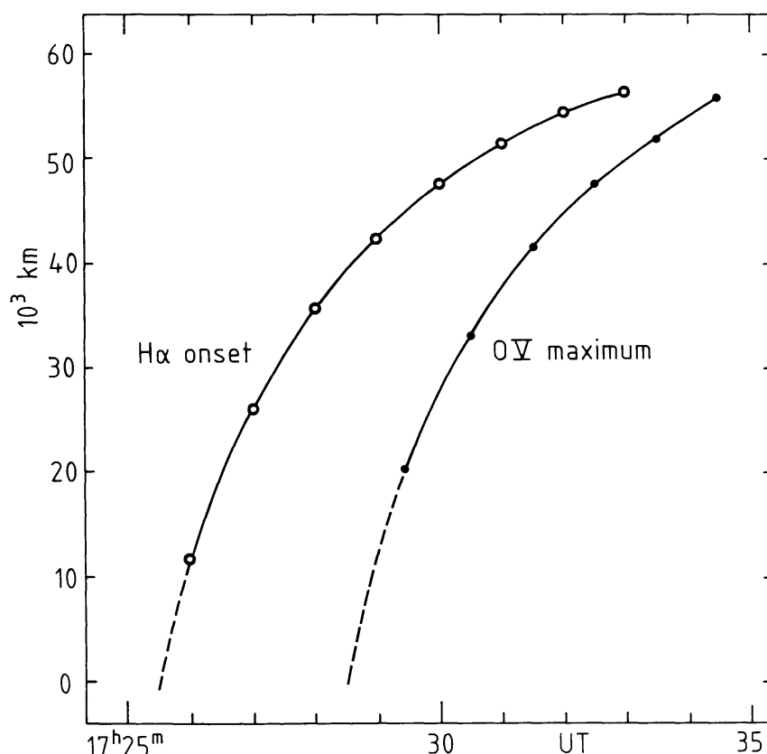
Fig. 11. Time of the H \alpha emission onset (i.e., position of the H \alpha leading edge, circles) and O v flux maximum (dots) at various distances from the primary footpoint of the SB arch (No. 18 in Table I). The H \alpha values have been taken from Table I of Paper I. The O v times are smoothed values based on the time of the highest maxima in Figure 10.
