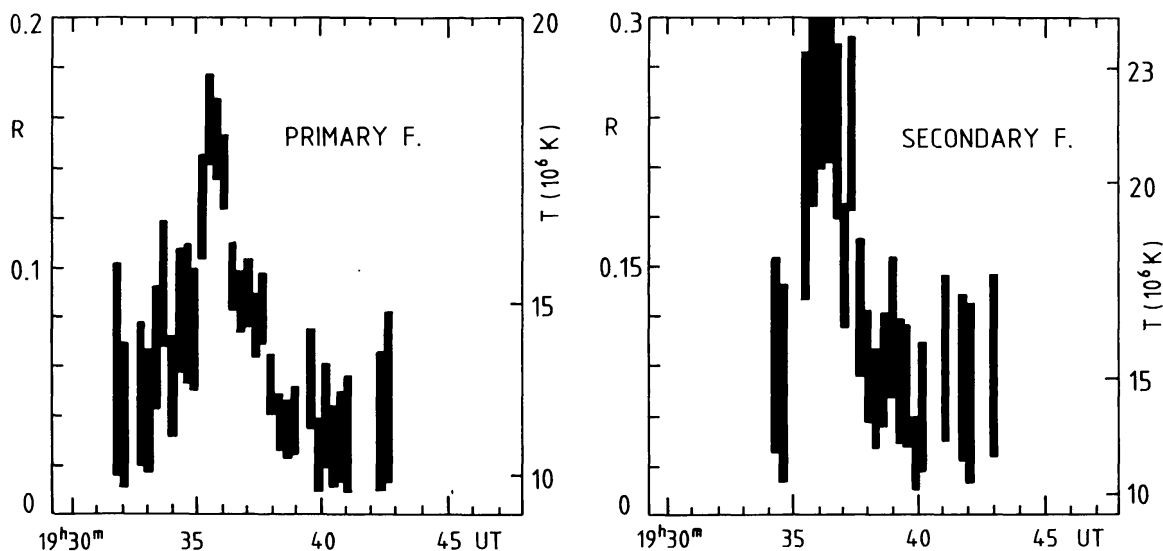
Fig. 8. Time development of the flux ratio (8.5–11 keV)/(3.5–5.5 keV) in the flaring arch No. 23. Left : primary footpoint; right : secondary footpoint. The right-hand scale gives the corresponding temperature for thermal emission after Mewe, Gronenschild, and van de Oord (1985).
