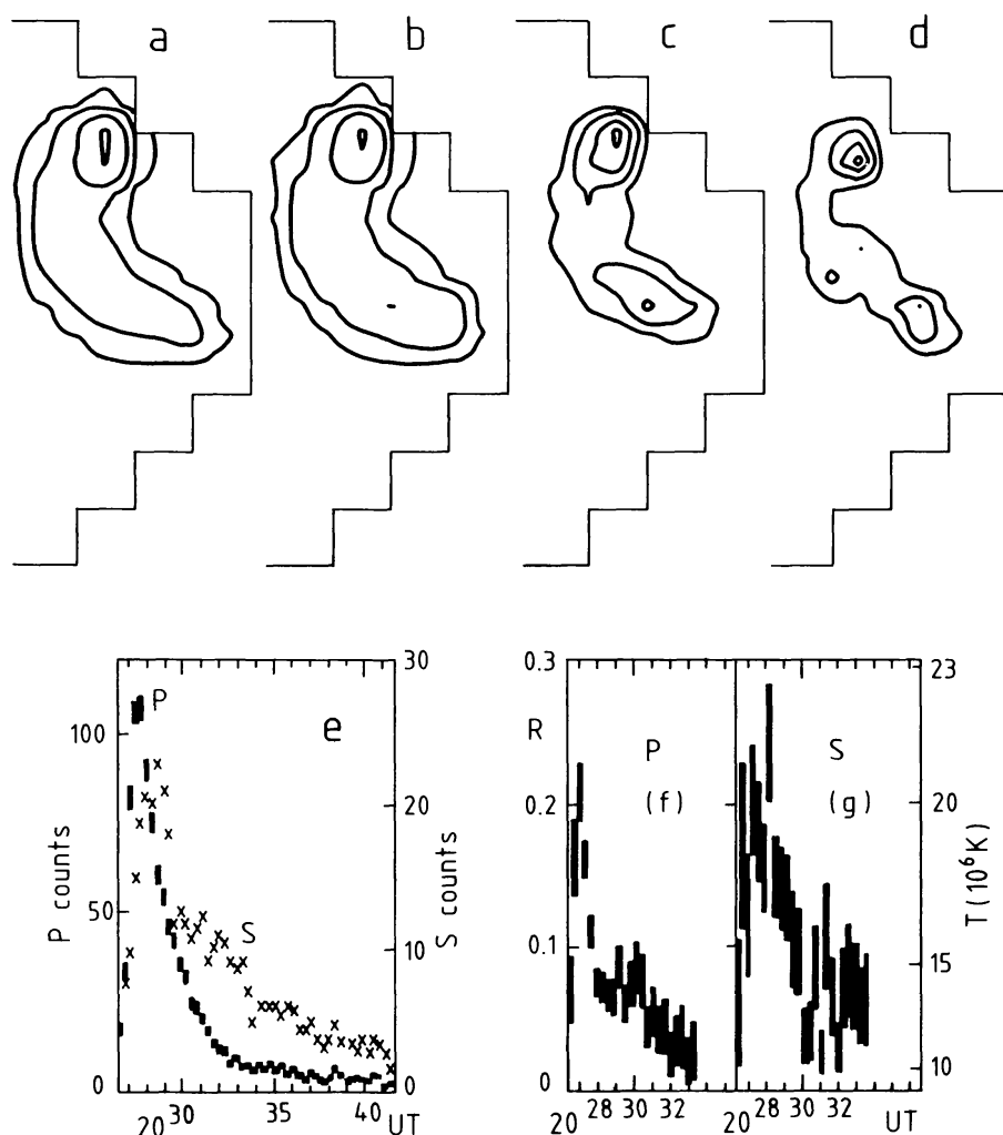
Fig. 9. The flaring arch No. 24 in Table I. (a)–(d) HXIS fine-field-of-view images at 20:28:47 ± 55 s UT: (a) 3.5–5.5 keV (max. 23.2 cts s -1 ); (b) 5.5–8.0 keV (max. 10.5 cts s -1 ); (c) 8.0–11.5 keV (max. 1.45 cts s -1 ); (d) 11.5–16 keV (max. 0.36 cts s -1 ). (e) Time development of the 3.5–5.5 keV X-ray emission at the primary ( P ) and secondary ( S ) footpoints. (f) and (g) Time development of the flux ratio (8.0–11.5 keV)/(3.5–5.5 keV) at the primary ( P ) and secondary ( S ) footprint. The right-hand scale gives the corresponding temperature for thermal emission after Mewe, Gronenschild, and van de Oord (1985).
