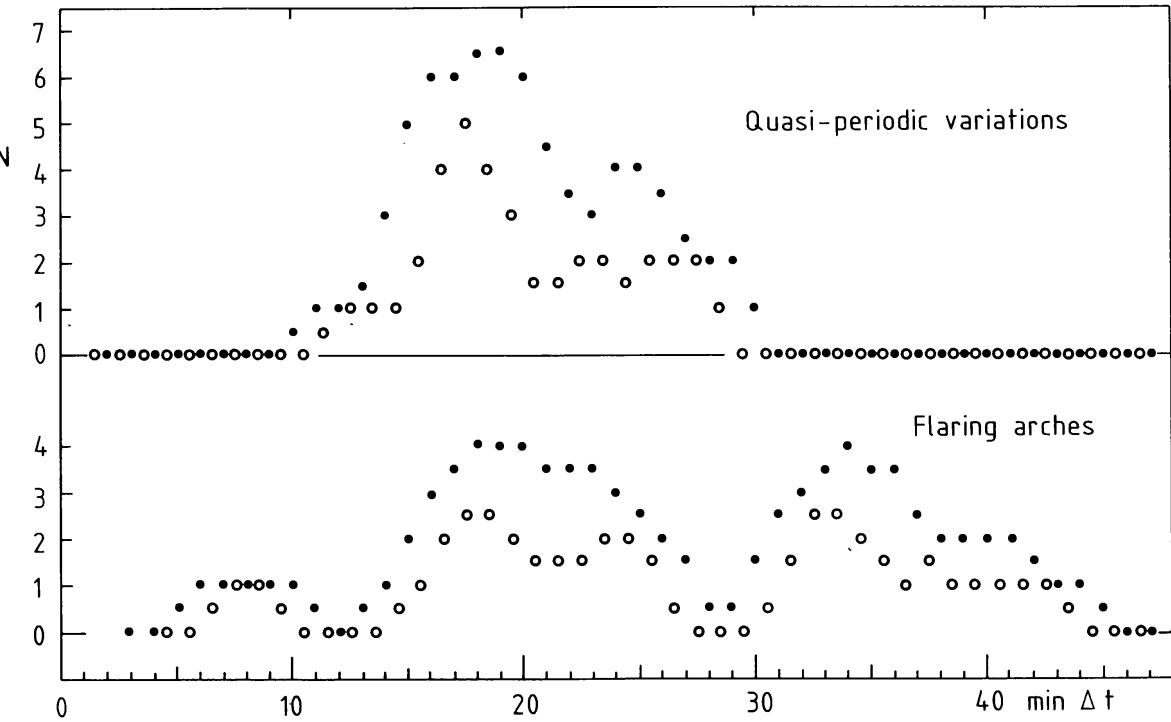
Fig. 4. Distribution of time intervals \Delta t between maxima of successive quasi-periodic variations ( above ) and onsets of successive flaring arches ( below ). Numbers N are smoothed values, with smoothing windows of 3 min (circles) and 6 min (dots). The real number of events was 13 for the variations and 17 for the arches.
