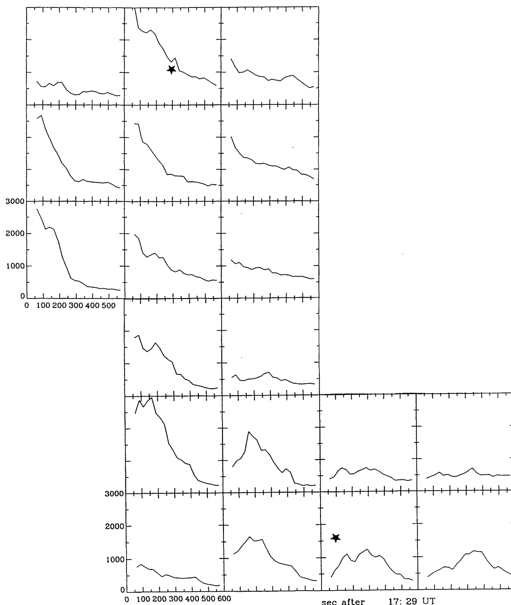
Fig. 10. Time development of the O v flux in individual pixels ( 10 \times 10 arc sec) during the SB arch (No. 18 in Table I). The O v flux has been read by the UVSP experiment every 27 s. The vertical (counts) and horizontal (time) scales are the same for all pixels though they are shown just for two of them. Approximate positions of the two footpoints are marked by asterisks. Note that the UVSP observations started only at 17:30 UT, 4.5 min after the onset time of the flaring arch in H \alpha and X-rays. North is up and west is to the right.
