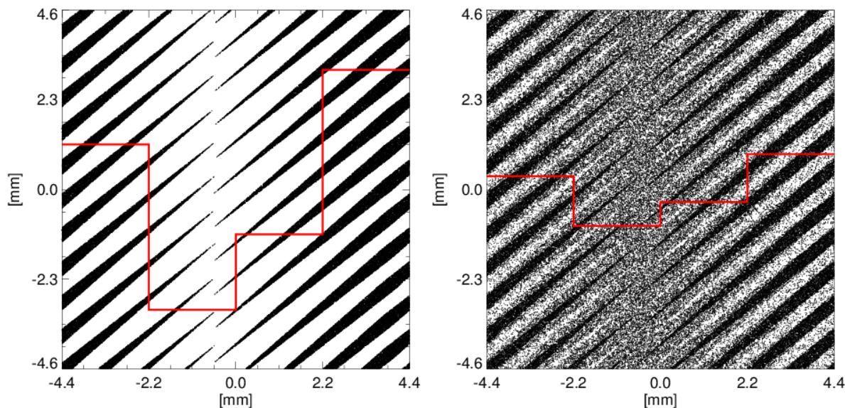
Moiré pattern from Geant4
