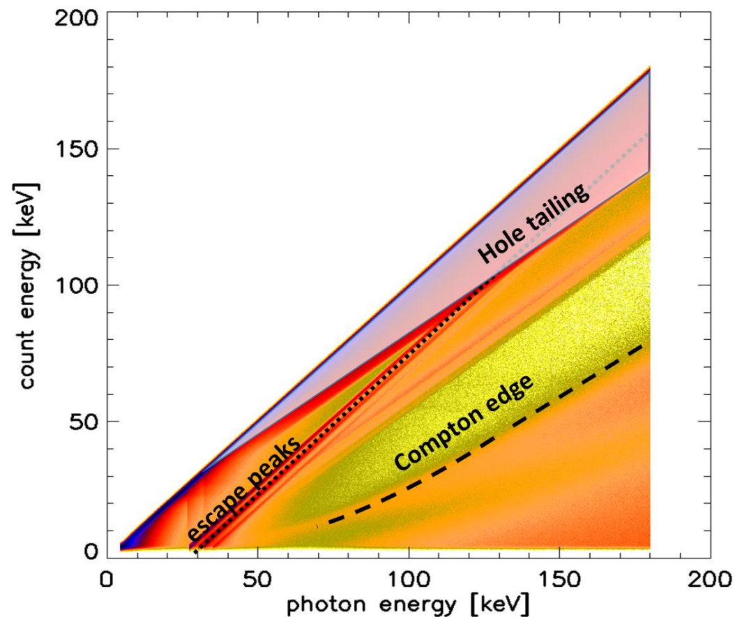
Detector Response Matrix (DRM)
