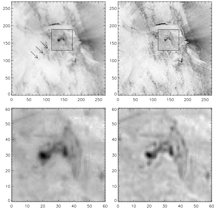
Figure 2. Top-left panel – a nonsaturated image of a compact EUV flaring event observed by TRACE in the 171 Å filter on October 21, 1999 at 19:54:43 UT with an exposure time of five seconds. The diffraction effects are visible up to sixth order in this image (three of the diffraction structures seen in the lower-left pattern arm are indicated by arrows in the image). Top-right – deconvolved TRACE image corresponding to the image from the top-left panel . The central image portions (in the boxes ) of both data and deconvolved frames are shown enlarged in the bottom-left and bottom-right panel , respectively.
