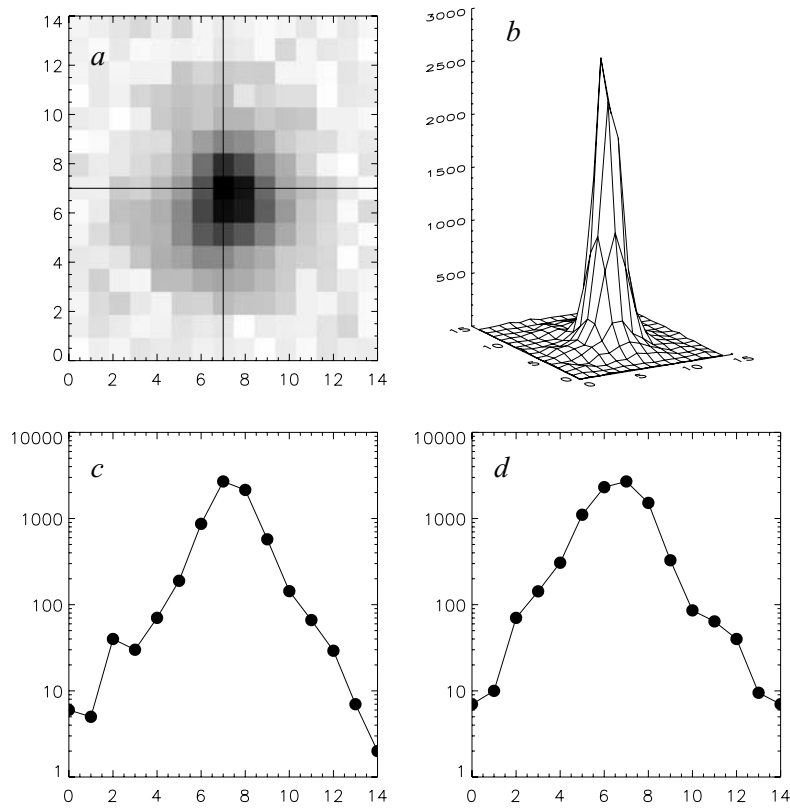
Figure 4. a: Enlarged image of the background-subtracted first-order maximum from the upper-left diffraction arm in Figure 1. b: Surface plot of the data from (a). c and d: Cross-sections of the maximum along the horizontal and vertical lines shown in (a).
