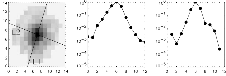
Figure 6. Left panel: Deconvolved TRACE PSF core. Middle and right panels: PSF core cross-sections along lines L1 and L2, respectively.
