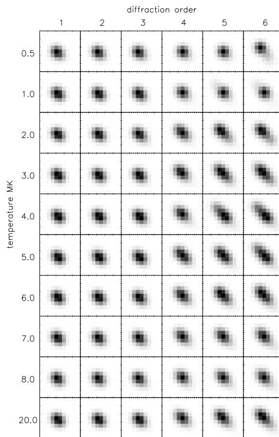
Figure 10. Temperature variability of the individual shape of the TRACE PSF diffraction structures (for orders 1–6) obtained in the isothermal approximation. Each individual structure was constructed using CHIANTI isothermal spectra multiplied by the TRACE effective area function, and convolved with the PSF core determined from blind deconvolution. The size of each small panel in this figure is 11 \times 11 TRACE pixels.
