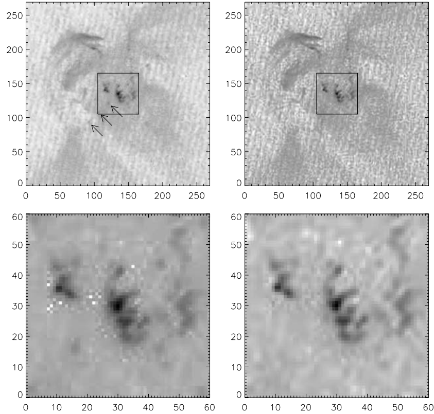
Figure 3. Top-left panel – a TRACE 171 Å compact flare image taken on June 19, 2001 at 09:56:46 UT with an exposure time of one second. The diffraction effects are visible up to sixth order in this image (three of the diffraction structures seen in the lower-left pattern arm are pointed to by arrows in the image). This image after deconvolution is shown in the top-right panel . The central portions of both data and deconvolved image (in the boxes ) are enlarged in the bottom-left and bottom-right panel , respectively.
