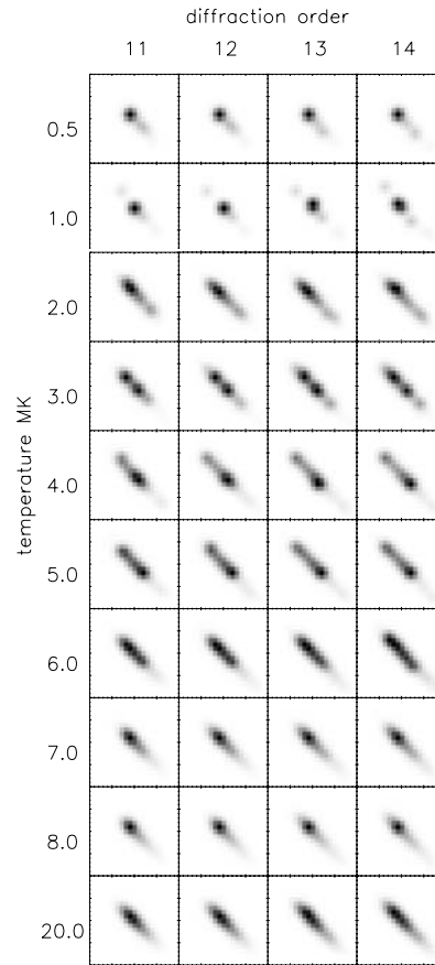
Figure 11. Temperature variability of the individual shape of the TRACE PSF diffraction structures (for orders 11–14) obtained in the isothermal approximation. Each individual structure was constructed using CHIANTI isothermal spectra multiplied by the TRACE effective area function, and convolved with the PSF core determined from blind deconvolution. The size of each small panel in this figure is 21 \times 21 TRACE pixels.
