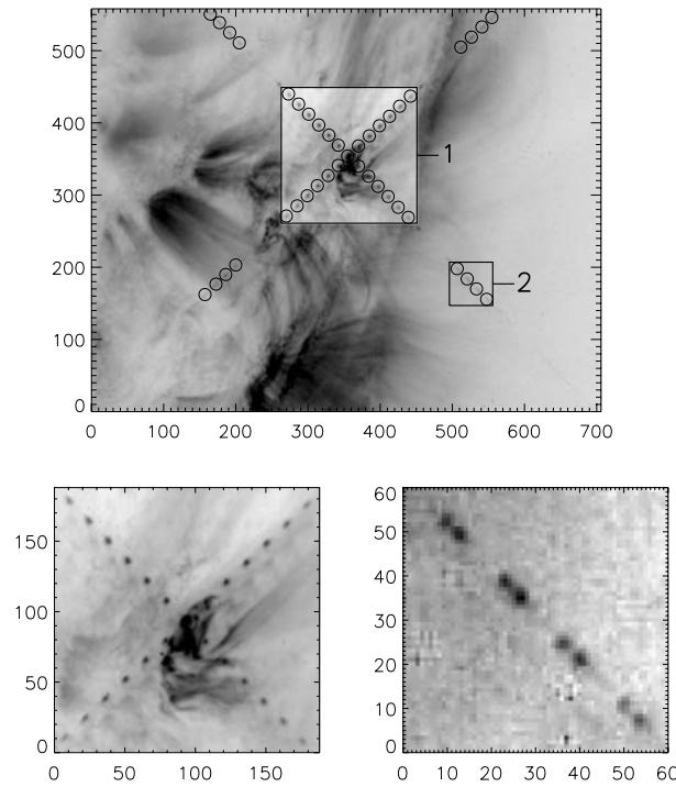
Figure 1. Top – TRACE 171 Å compact-flare image taken on May 16, 1999 at 13:49:22 UT with an exposure time of 19.5 seconds. The TRACE PSF maxima are clearly visible extending outwards in four arms from the saturated flaring area. Encircled are the stronger maxima of orders 1–6 and 11–14 which are investigated in more detail in the present study. For presentation purposes, different signal scaling was used for the image portion in box 1 containing maxima up to sixth order. This portion is shown enlarged in the bottom-left panel. The sub-image in box 2 with further diffraction structures of orders 11–14 is expanded in the bottom-right panel.
