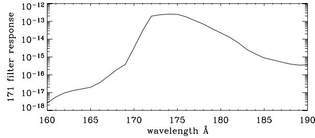
Figure 8. Spectral response curve for the TRACE 171 Å filter. The curve is given in units of \text{DN cm}^2 \text{sr photon}^{-1} \text{pixel}^{-1} .
