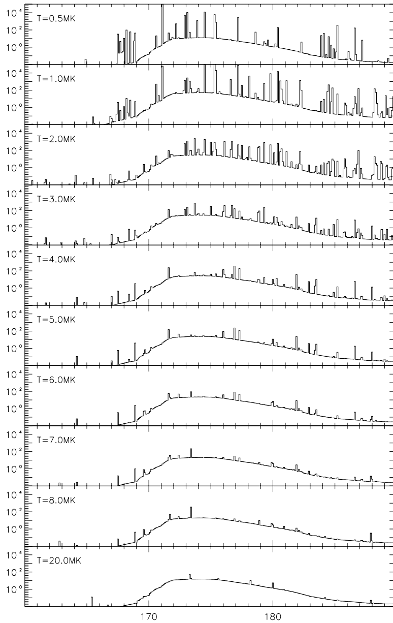
Figure 9. Isothermal spectral contribution functions to the TRACE image signal as calculated for a range of temperatures. The units on the y-axes of the plots are \text{DN s}^{-1} \text{pixel}^{-1} .
