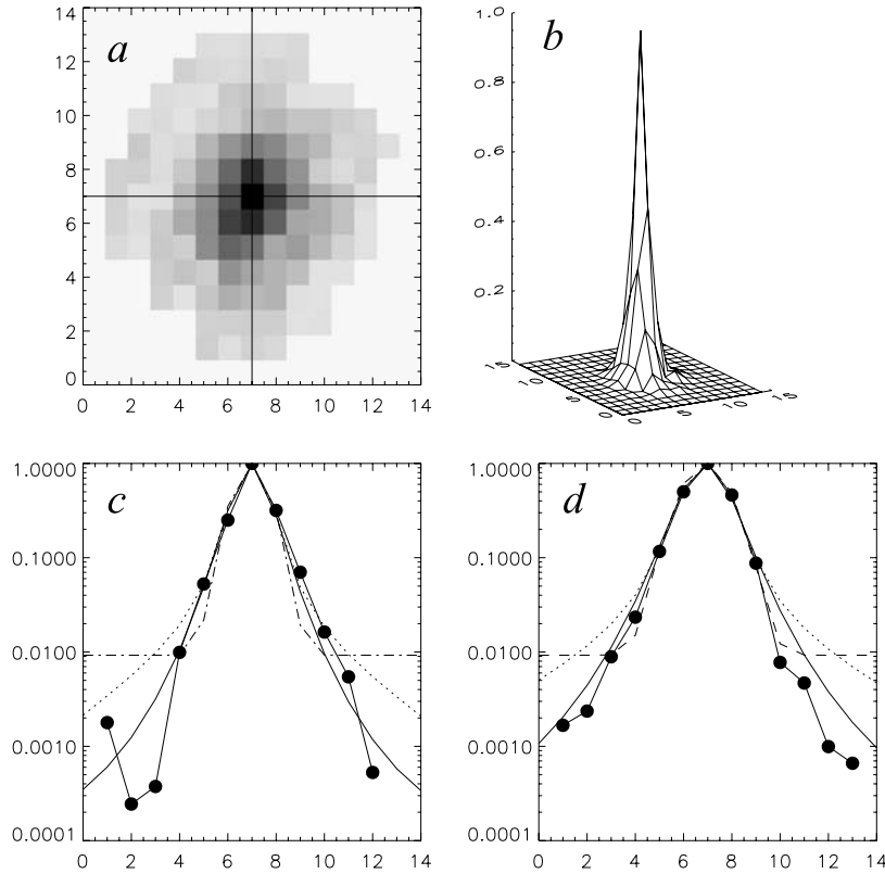
Figure 7. Image of the deconvolved TRACE PSF core (a) and its surface plot (b). In (c) and (d) the cross-sections of the peak along the horizontal and vertical lines in (a) are plotted. The PSF core cross-sections are plotted as a thick solid line with black dots . The corresponding cross-sections of the best fits to the core in terms of analytical functions are overplotted in (c) and (d). The Moffat function fit cross-sections are plotted in a thin solid line , for the Gaussian fit a dash-dotted line is used, and for the fit of the Voigt profile – the dotted line .
