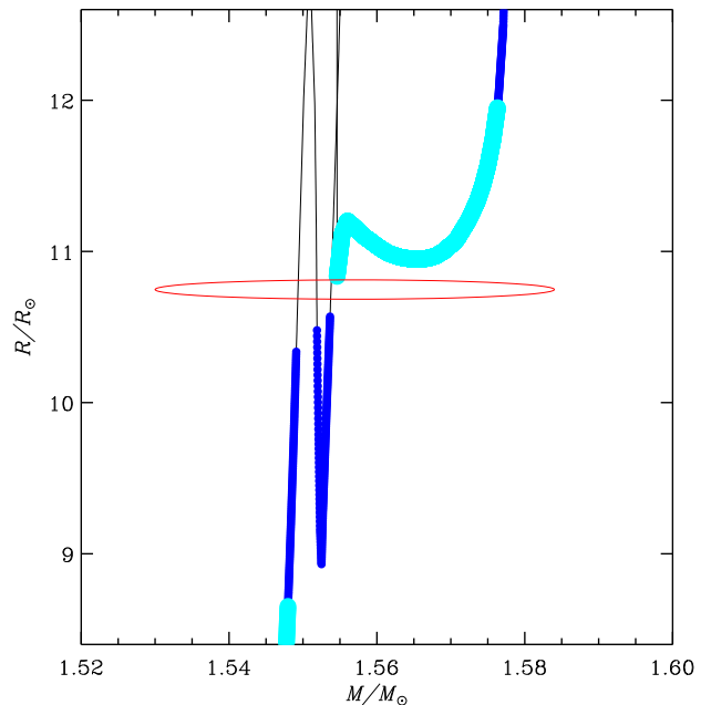
Fig. 8. Zoom on the upper part of Fig. 7. The isochrone is coloured cyan or blue in regions where the isochrone T_{\text{eff}} is within 0\text{--}1\sigma or 1\text{--}2\sigma , respectively, of the measured T_{\text{eff}} of the RG.
