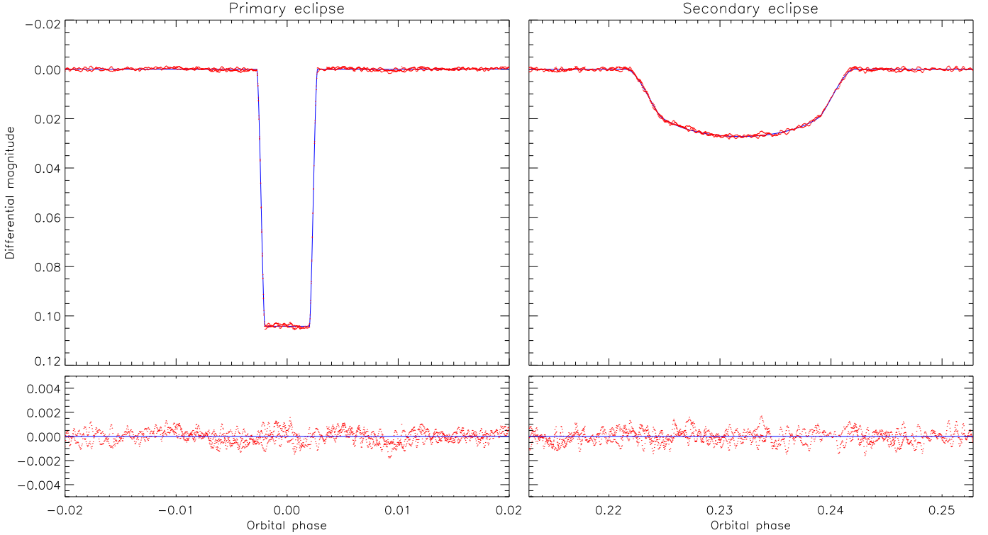
Fig. 6. The primary (left panels) and secondary eclipse (right panels) of KIC 8410637. The Kepler data points are shown as red dots and the JKTEBOP best fit as the blue curve. The residuals of the fit are shown in the lower panels with an expanded scale on the ordinate axis.
