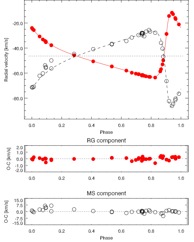
Fig. 5. Plot of the SBOP solutions for the two components of KIC 8410637. Red dots are for the RG, open black dots for the MS star. Note the difference in vertical scale for the O-C plots.
