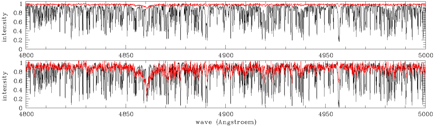
Fig. 4. Decomposed spectra of the RG (black) and the MS (red) star in the H\beta region. Top: Normalised to the common continuum of both components. Bottom: Normalised to the continua of the single components.
