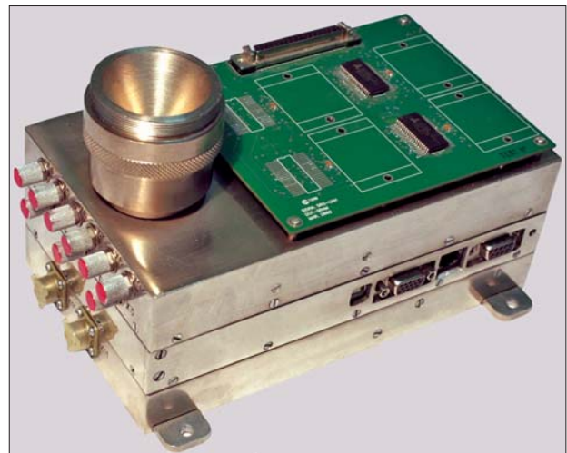
Fig. 1. Overall view of the of the SIDRA device breadboard model
