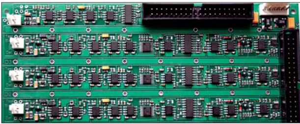
Fig. 3. General view of the signal analog processing channels of printed board from the side of component mounting
