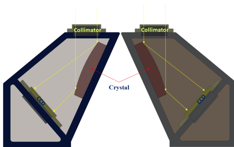
Spectrometer System
