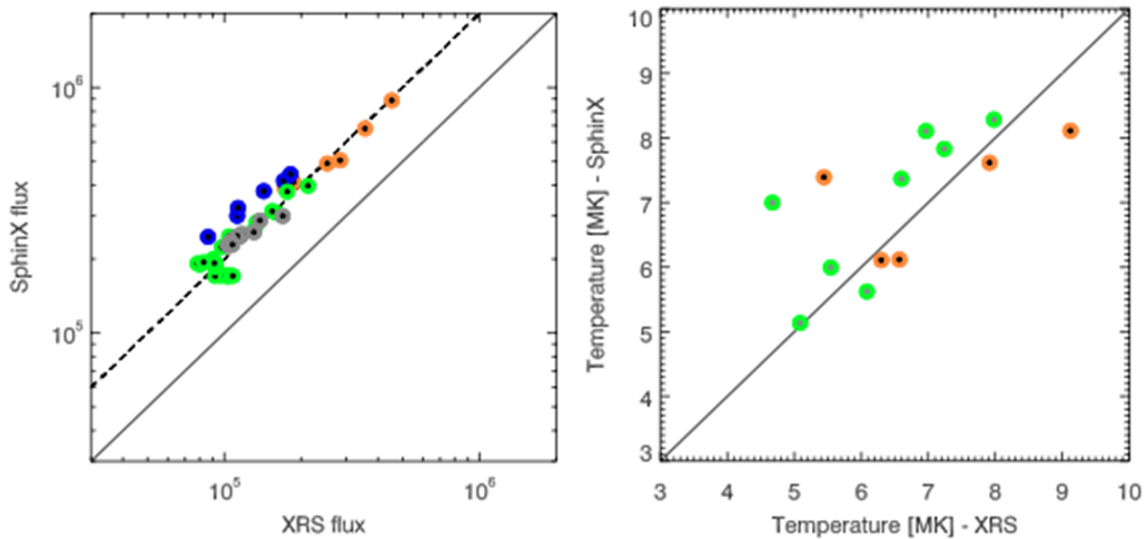
Fig. 9. Comparison of XRS (MESSENGER) and SphinX absolute fluxes of solar X-ray emission above 1 keV (left). SphinX values are about twice those of the XRS, though the derived plasma temperatures (from an isothermal assumption) are in a good agreement. Different colours correspond to particular small flares indicated by arrows in Fig. 8 (lower panel).
