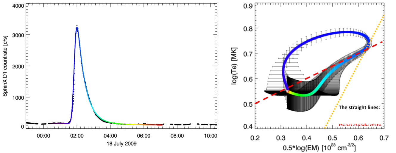
Fig. 7. Example of the elementary flare time profile fits with the SphinX light curve of a small (A9.0) event SOL2009-07-18T0204 (left) and the corresponding diagnostic diagram (right) showing the evolution of the plasma emission measure and the temperature. Changing colours reflect progressing times. It is observed that the initial decay phase runs along the steady state branch (red dashed). At later times the “heating-OFF” takes place and the inclination steepens, being close to the OFF-case (yellow dot branch). Such a detailed study has been performed for the first time and the results are to be presented in a dedicated paper.
