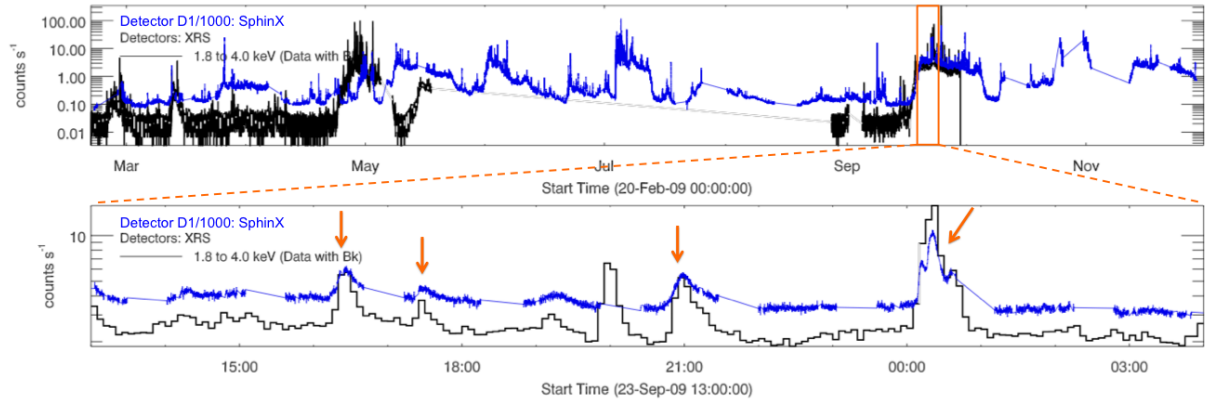
Fig. 8. Upper panel: The comparison of X-ray lightcurves of the Sun as seen from MESSENGER (black) and SphinX (blue). The sensitivity of SphinX was many times higher than XRS. For the period in late September 2009 (lower panel), MESSENGER observed the same part of the solar disk, so a direct comparison is possible.
