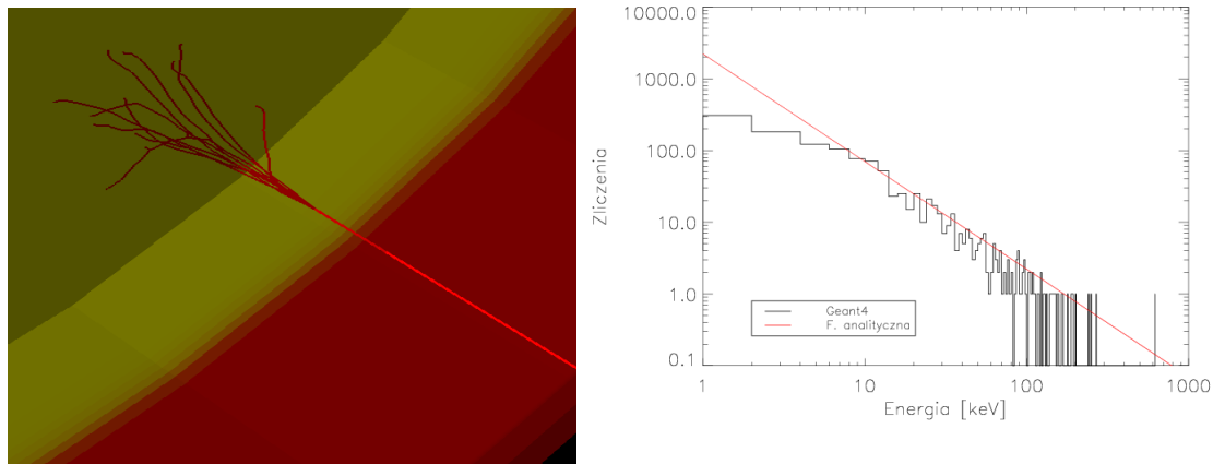
Fig. 11. Left: the visualization of the relativistic electron track (red) impeding the solar denser chromosphere. Secondary electron paths are clearly visible leading to emission of the bremsstrahlung continuum. Right: Spectrum of X-ray emission calculated using Geant4 for the electron power low beam above 10 keV (histogram). Straight line represents the analytical solution.
