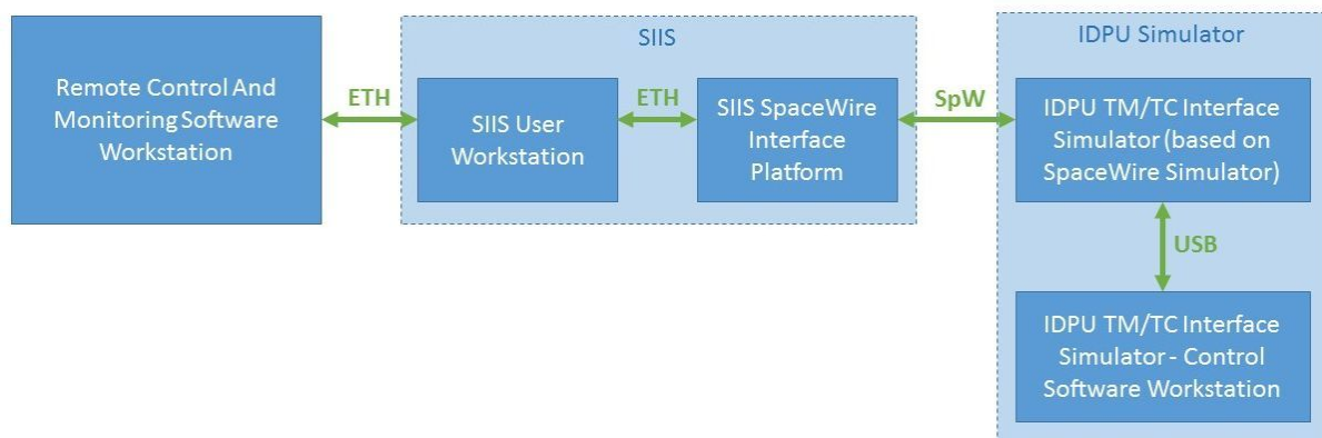
Fig. 13. Block scheme of the STIX test configuration to be used for EM and FM of the instrument.
