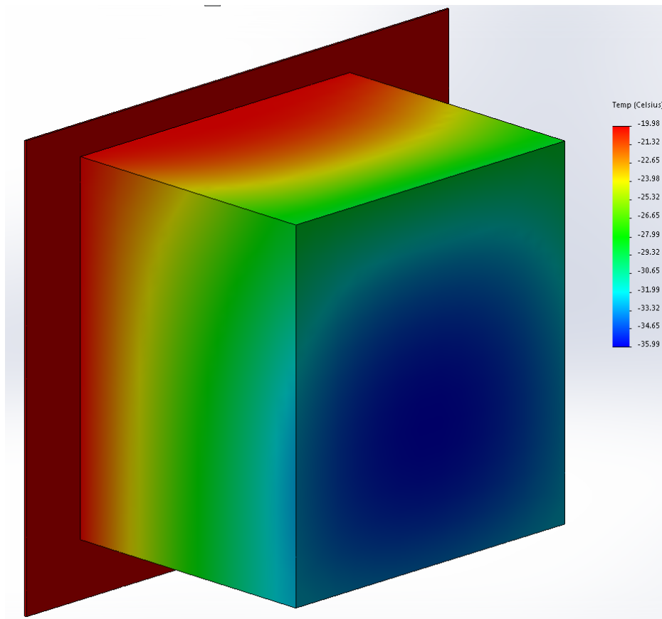
Fig. 16. Distribution of ChemiX instrument temperatures, calculated for the case of the instrument support temperature being at -20 C. This corresponds to the lowest temperature envisaged for the payload support plate.
