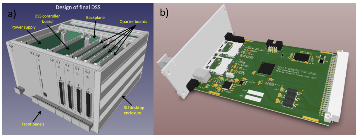
Fig. 12. A view of the detector simulator system (DSS-left) and one of the printed boards to be placed inside.
