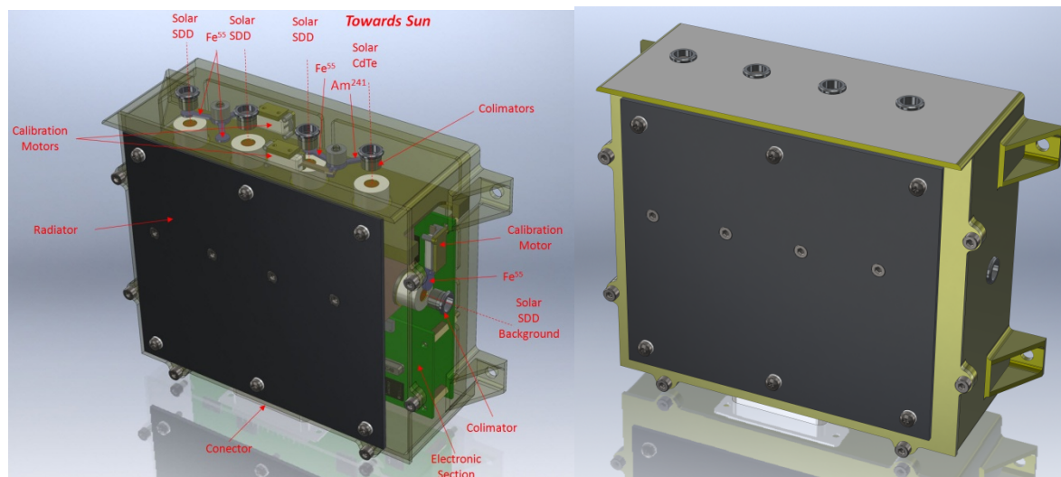
Fig. 19. The construction of SphinX-NGP soft X-ray spectrophotometer intended to be placed on the front satellite (occulter) of the Proba-3 formation flying duo.
