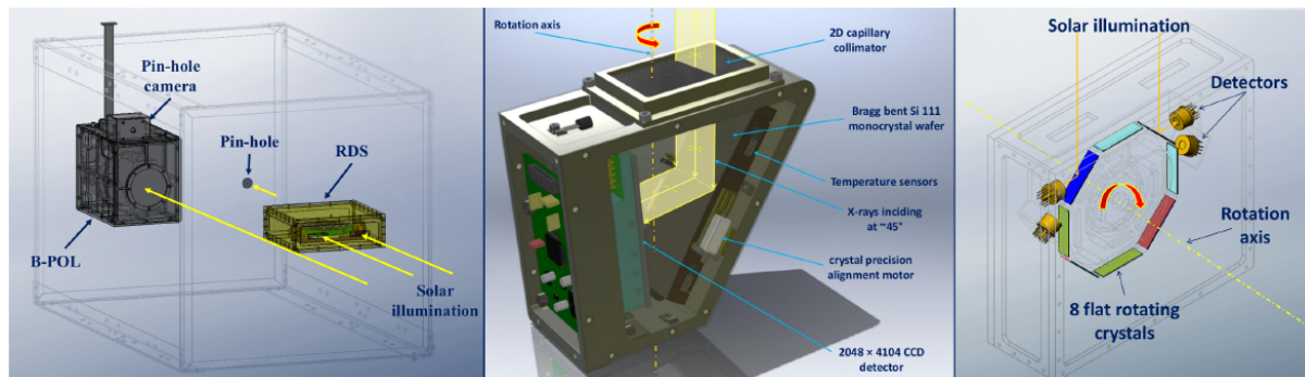
Fig. 17. A view of the three SolpeX units within KORTES shadow. The B-POL rotating polarimeter axis is actively directed towards the flare (being in progress) as seen in the pin-hole image. The RDS consists of 8 flat crystals mounted on the rotating drum revolving 10 times/sec. Bragg-reflected X-rays are collected by four SDD detectors. Appropriate crystal selection assures a full spectral coverage over the soft X-ray spectral range.
