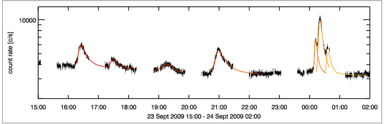
Fig. 6. Example of the fit to the observed lightcurve over a several-hour period of solar X-ray emission ( E > 1 keV) with individual elementary flare profiles.
