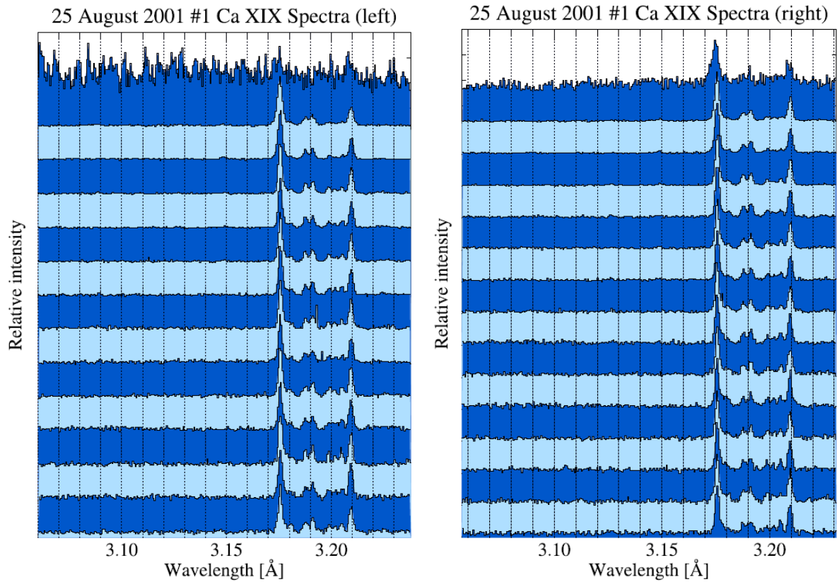
Fig. 5. Left: Forward (increasing wavelength) scans for DIOGENESS channel 4 (Ca XIX lines) during the 25 August 2001 flare stacked with increasing times from top to bottom (time range 16:29 – 18:00 UT). Right: Corresponding backward (decreasing wavelength) scans.
