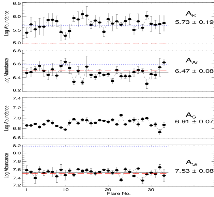
Fig. 4. Mean abundance estimates for each of the 33 flares of K, Ar, S, and Si. The red dashed horizontal lines indicate photospheric abundance estimates from Asplund et al. (2009) (Si, S, K) or solar proxies from Lodders (2008) (Ar). The blue dotted lines are coronal abundance estimates from Feldman et al. (1992), those specified in the CHIANTI database “coronal” abundance set.
