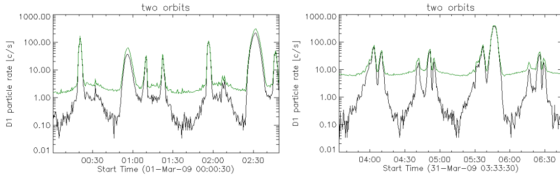
Fig. 10. Two examples of D1 SphinX records from the very low activity period. Green lines represent signal before “cleaning” and black after rejection of solar “events”. The dynamic range of the signal due to energetic particles is increased by about a factor of 100.
