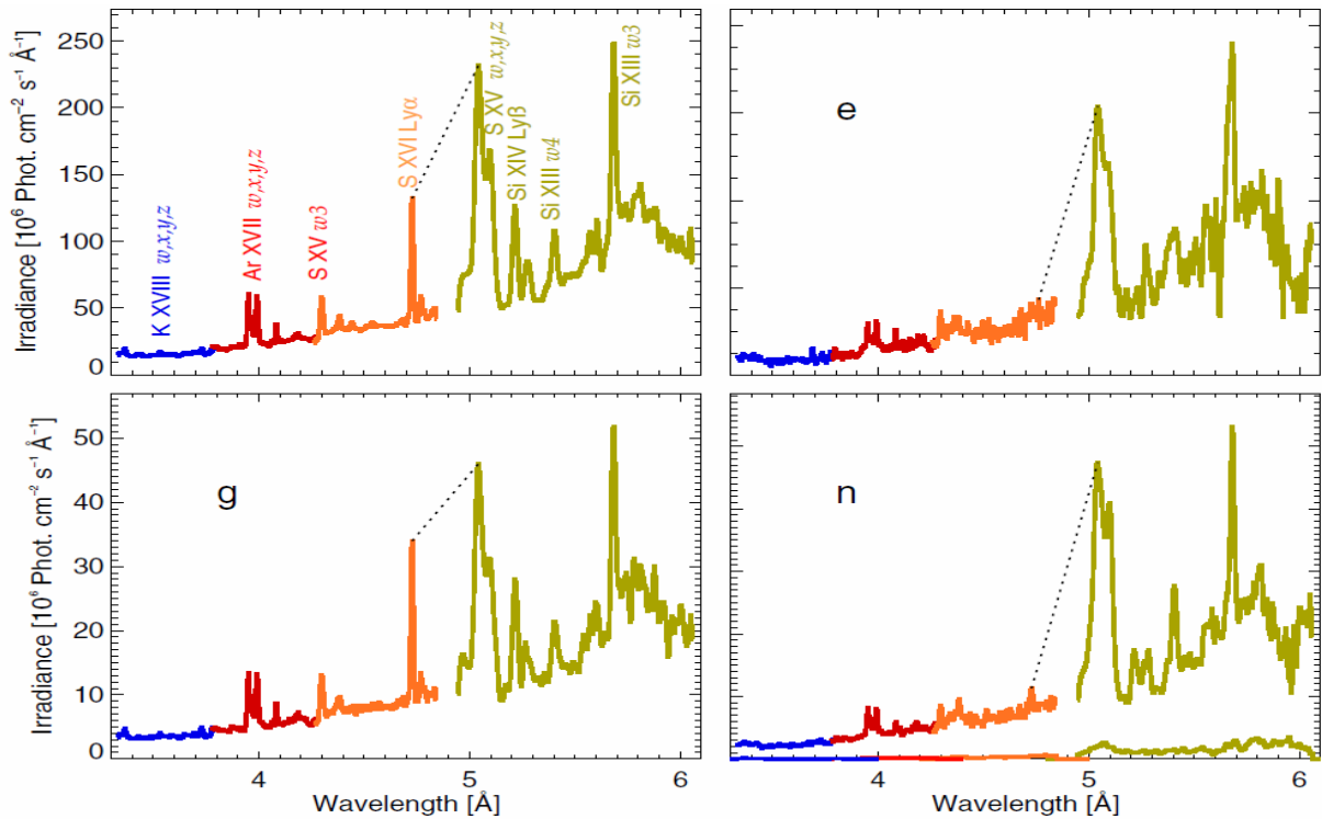
Fig. 1. Example of RESIK spectra for flare SOL2002-11-14T22:2. On the flare- averaged spectrum (top left panel), identifications of stronger spectral lines are given. Panels e, g and n correspond to the rise, maximum and decay phases of the event. The pre-flare spectrum is shown at the bottom of panel n.
