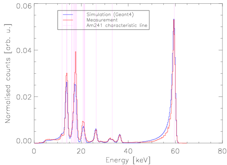
Fig. 14. Comparison of the measured STIX detector response (in red) with the Geant4 calculated response (in blue). Satisfactory agreement is observed. All 32 STIX detectors (flight units) will be measured and fitted in order to properly convert the stream of telemetry data into images of X-ray flares in selected energy ranges.
