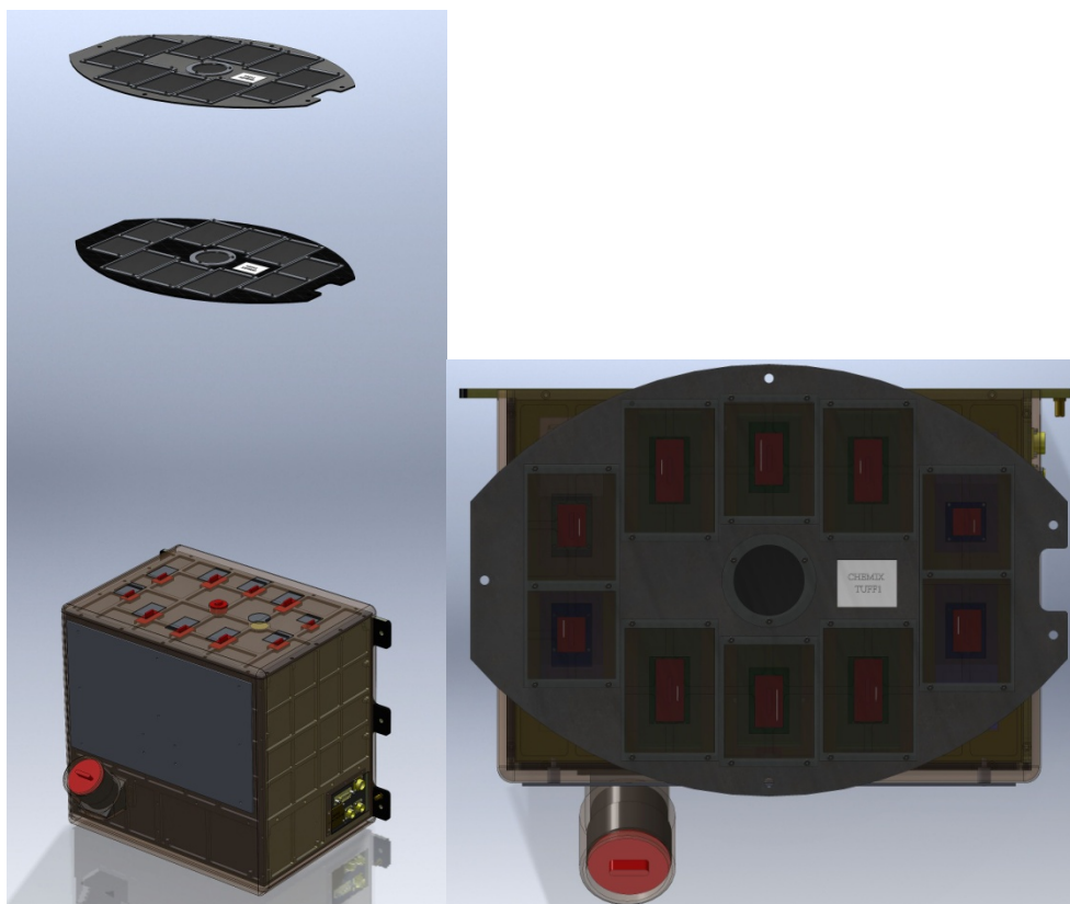
Fig. 15. General view of the ChemiX Bragg spectrometer (left). The upper two panels are the filter boards to be mounted on the mission thermal screen. They have to withstand harsh thermal conditions ( \sim 400 C). The crystals and detectors are mounted within the block placed \sim 1 m behind the filters. The red-capped tube is the particle detector system, under development by the Ukrainian Kharkiv group led by Dr. Dudnik. Right: a view of ChemiX from the direction of the Sun.
