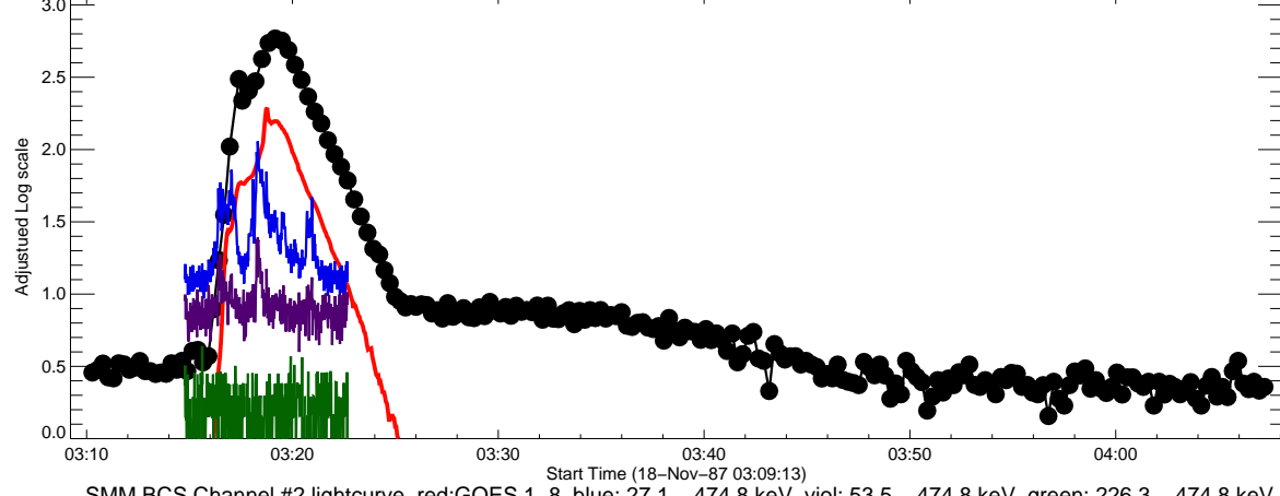
SMM BCS Channel #2 lightcurve red:GOES 1-8 blue: 27.1 - 474.8 keV viol: 53.5 - 474.8 keV green: 226.3 - 474.8 keV
