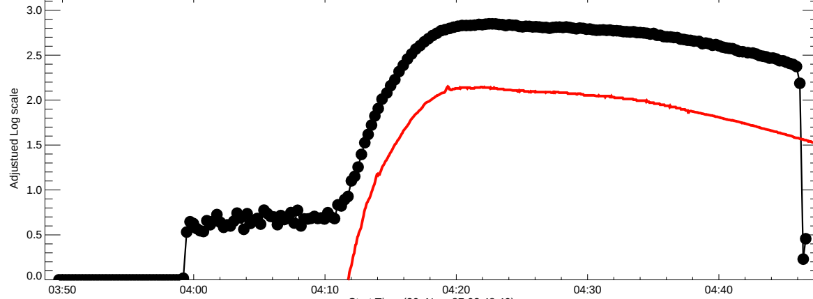
SMM BCS Channel #2 lightcurve red:GOES 1-8 blue: 27.1 - 474.8 keV viol: 53.5 - 474.8 keV green: 226.3 - 474.8 keV
