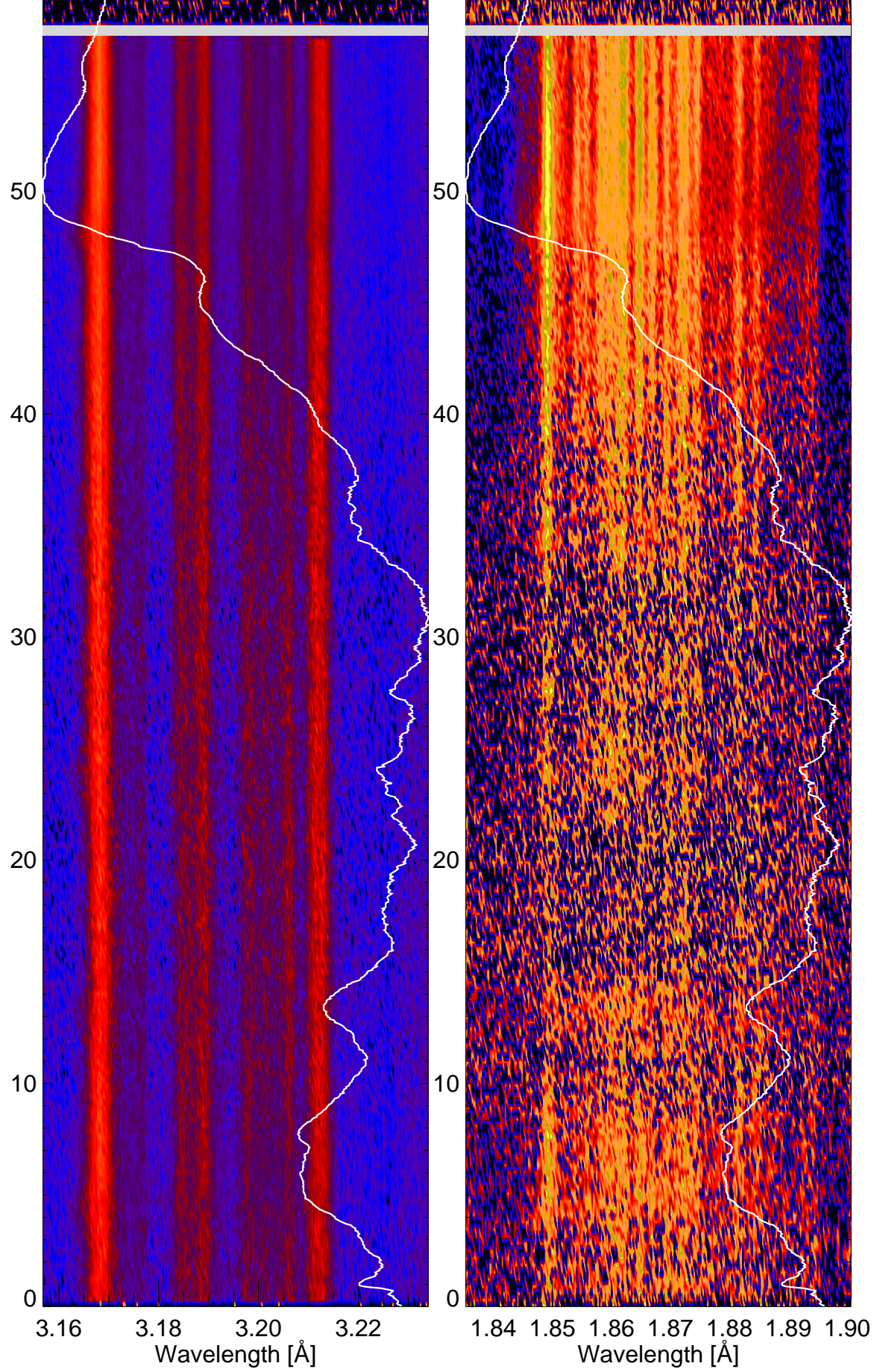
SOL_1989_Mar_13_13_15_32
