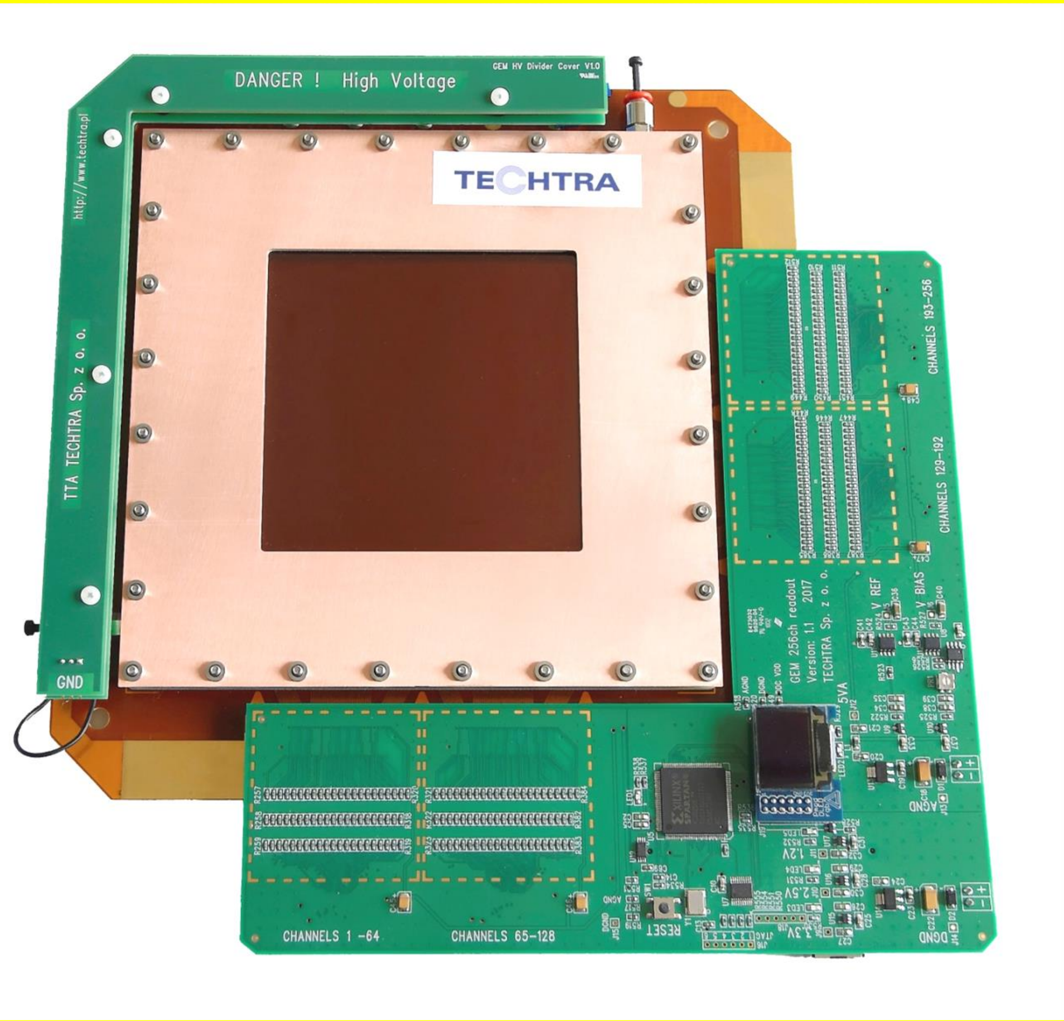
10 x 10 cm GEM detector with 256 ch V1.1 electronic readout
