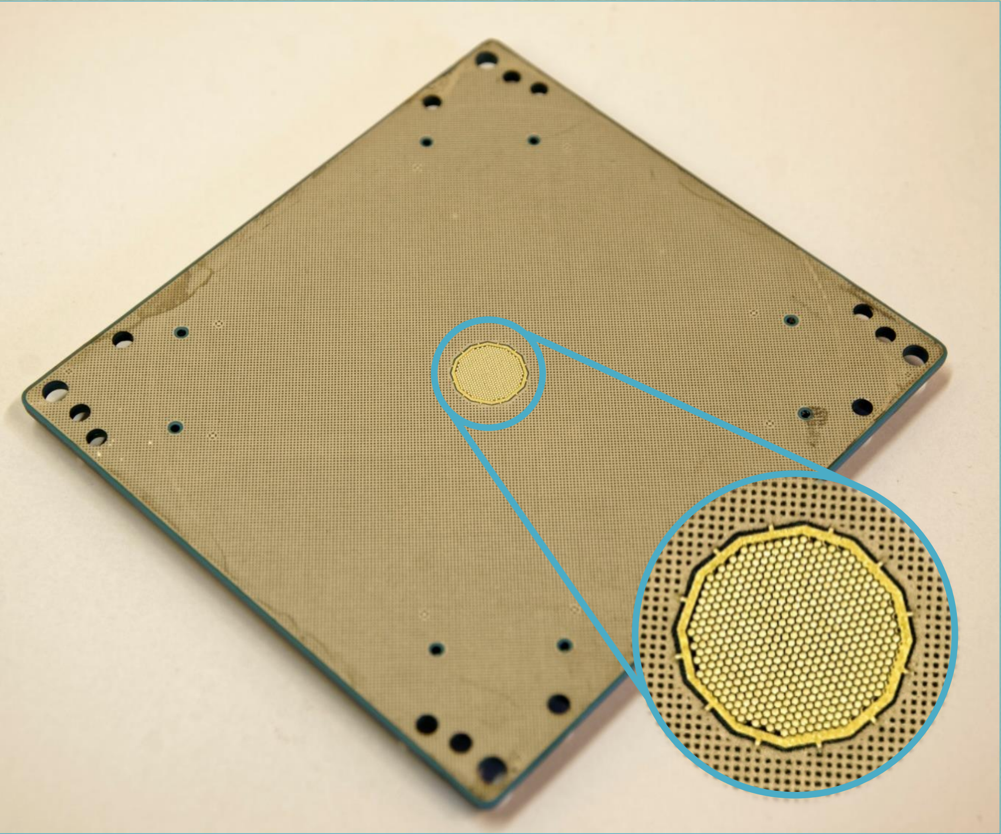
Hexagonal pad readout board
