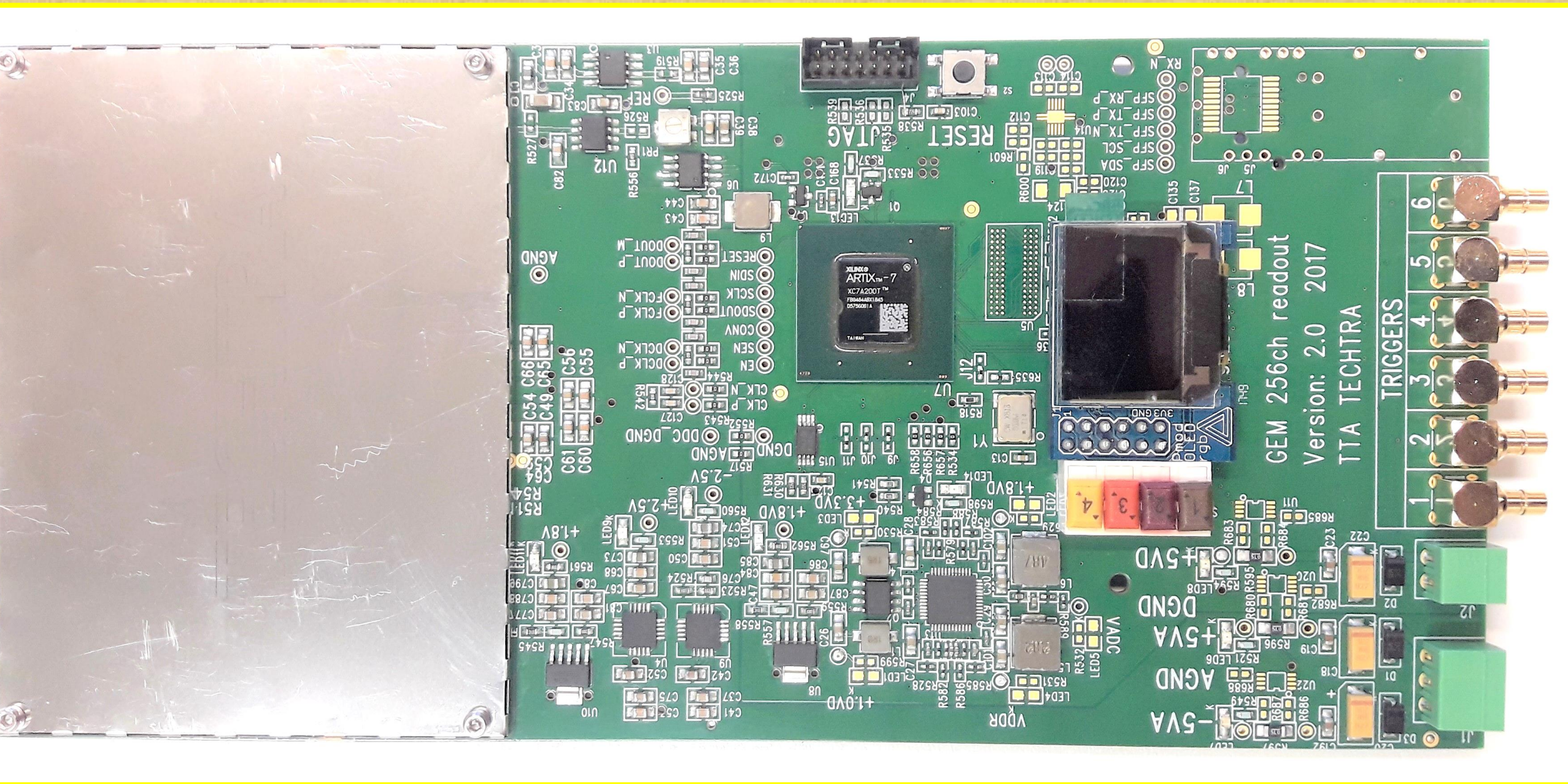
V2.0 electronic readout board
