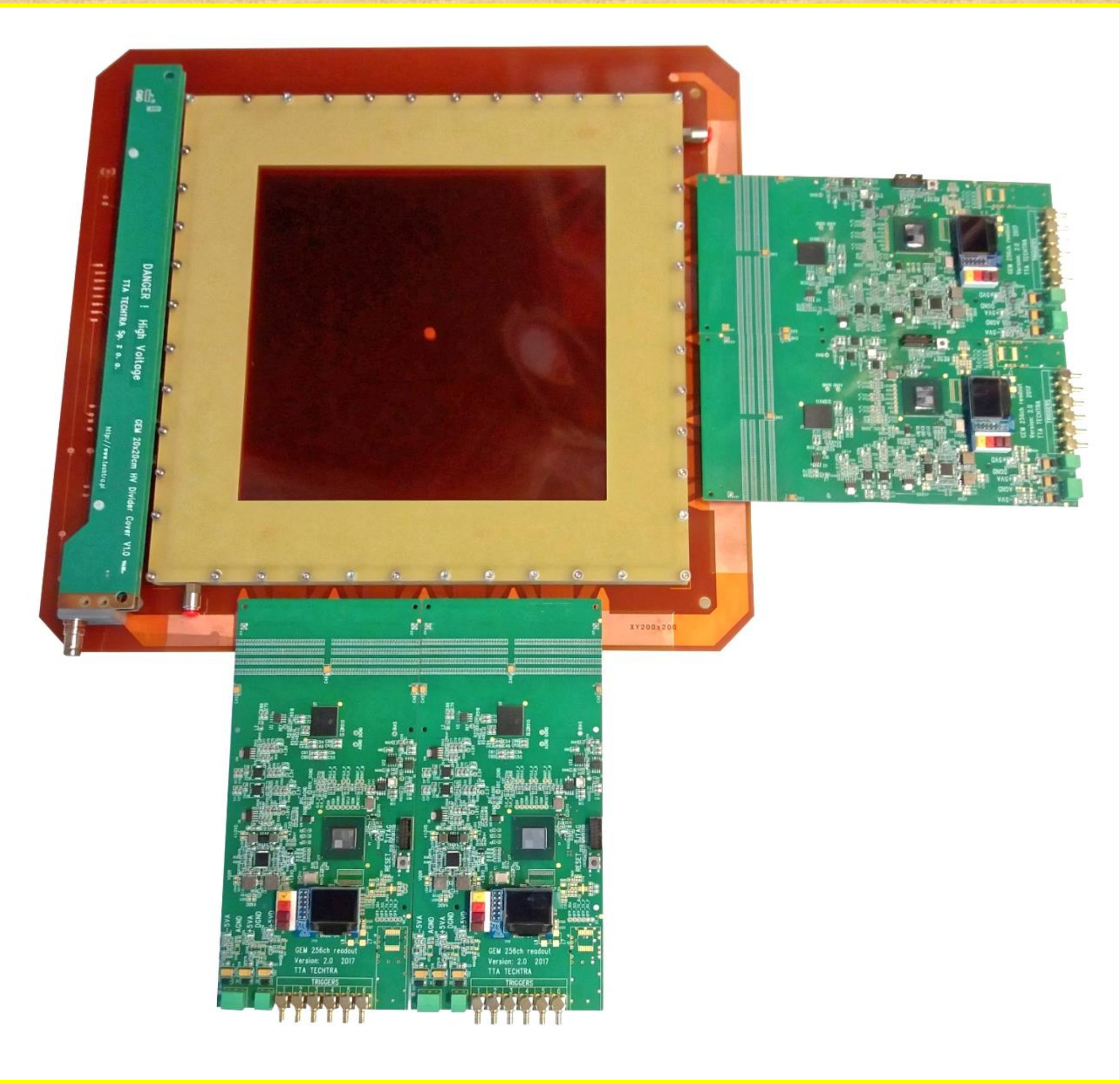
20 x 20 cm GEM detector with 4 x 256 ch V2.0 electronic readout
